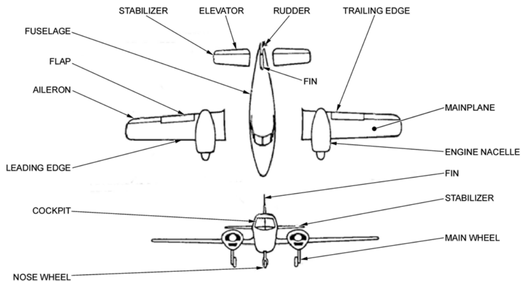
Figure 12-2-1 Airplane Components
