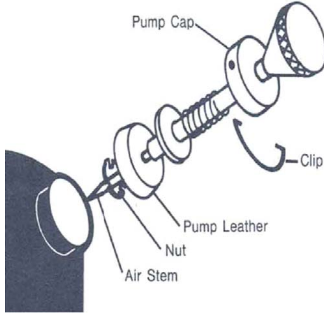
Figure 12 Pump Assembly
